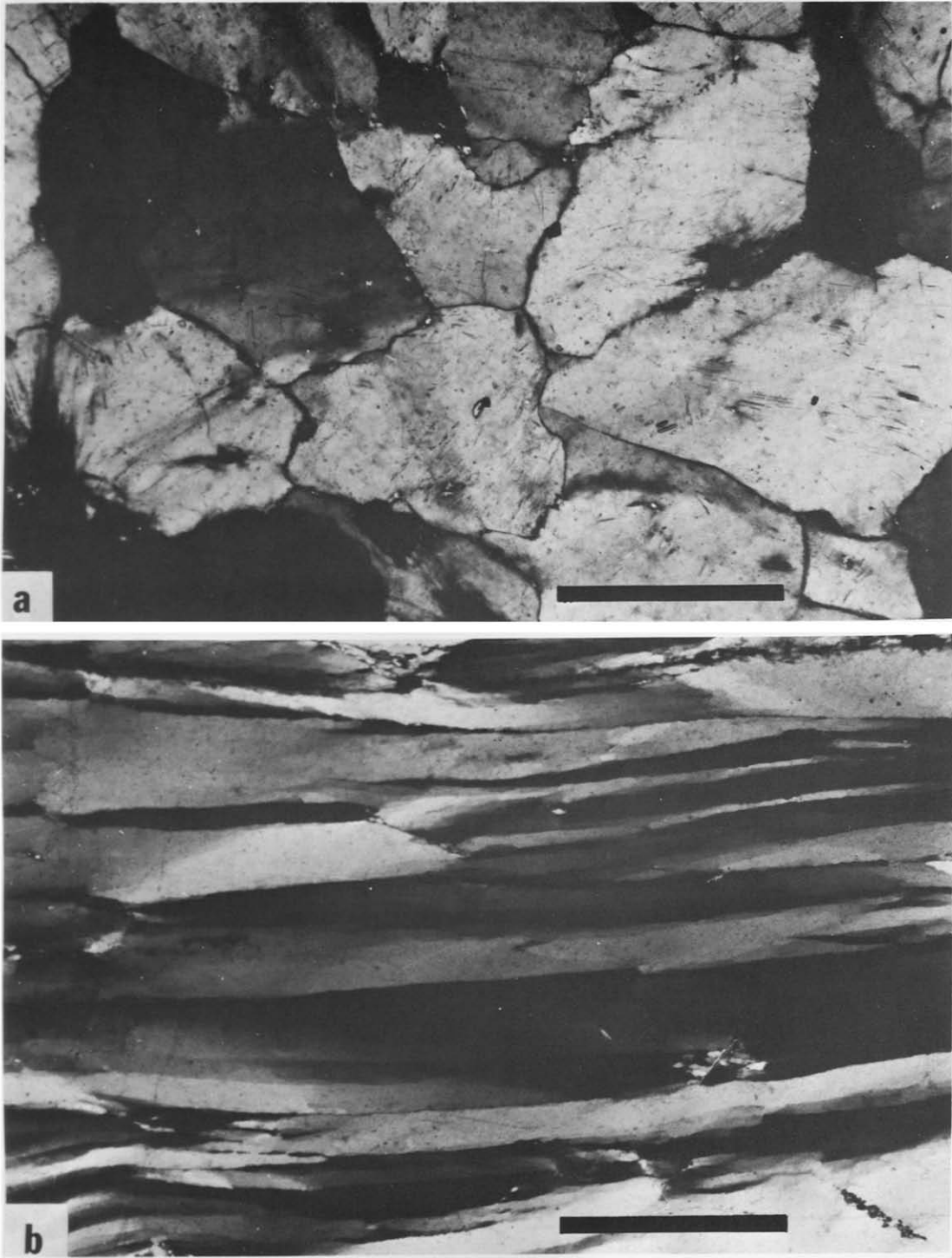
Fig. 3. (a) Photomicrograph of the less-deformed quartzite, perpendicular to the mineral lineation. A weakly developed foliation trends horizontally. Scale bar is 5 mm. (b) Photomicrograph of the quartzite mylonite, sample 506, perpendicular to the stretching lineation. Scale bar is 1 mm.
